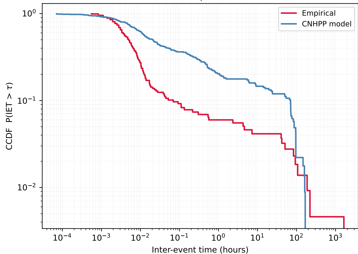
User 1457424889 - Empirical vs CNHPP model
